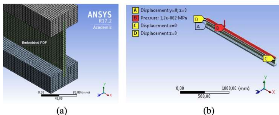
Figure 13: Numerical model of I-beam (a) Mesh; (b) Analysis parameters. Reproduced from (Kanócz et al. 2020) under CC-BY licence.
