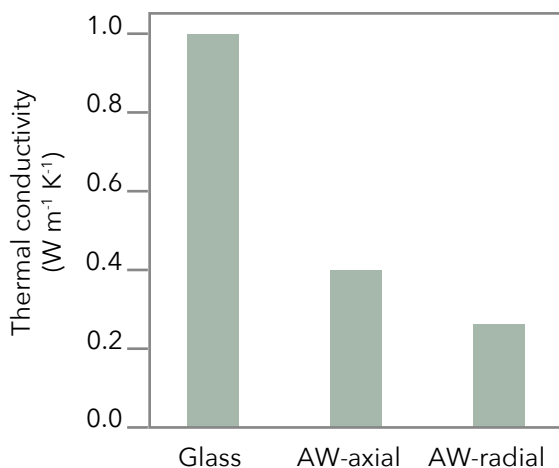
Figure 8: Thermal conductivities of “standard” glass and aesthetic TW (both considering axial and radial wood cut). Adapted from Mi et al., 2020 under CC-BY licence.
